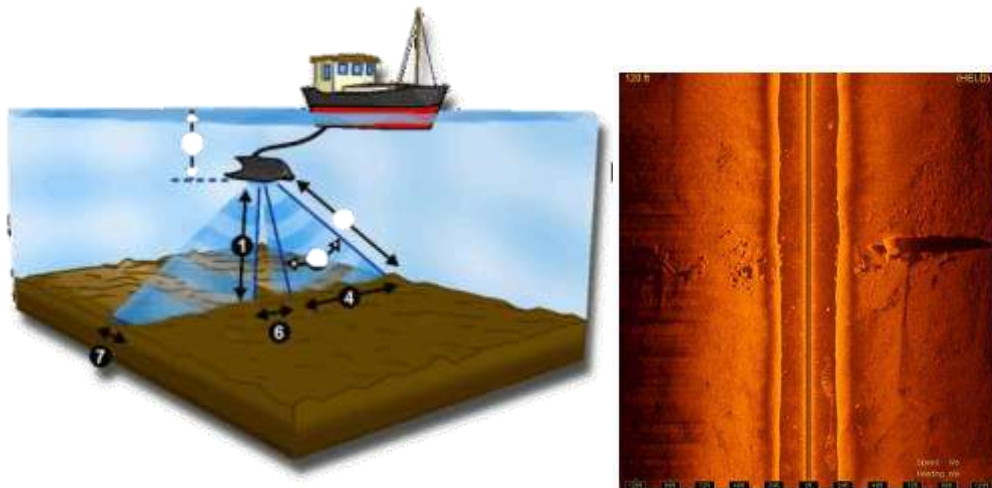
Figure 5. Side Scan Sonar (SSS)
